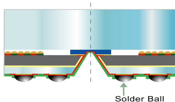
Step E: Passivation coating and BGA formation
